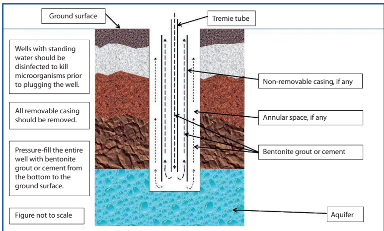
Figure 3. Plugging a well with bentonite grout or cement using a tremie tube.
