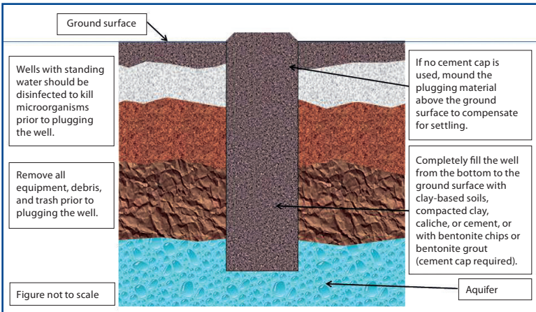
Figure 1. Plugged large-diameter well.
