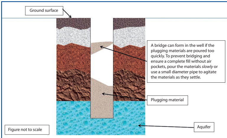
Figure 4. Bridging within a small-diameter well.
