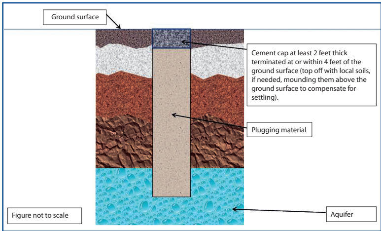
Figure 2. Well plugged with bentonite chips or bentonite grout.
